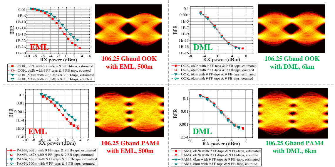
Fig. 2. BER results as a function of received (Rx) optical power for both 106.25 Gbaud NRZ-OOK and PAM4 for both the EML and the DML configurations, respectively. For each case the counted BER and estimated BER are shown to cover the full power sweep range. Selected eye diagrams at highest Rx power level after transmission are shown for all cases.
