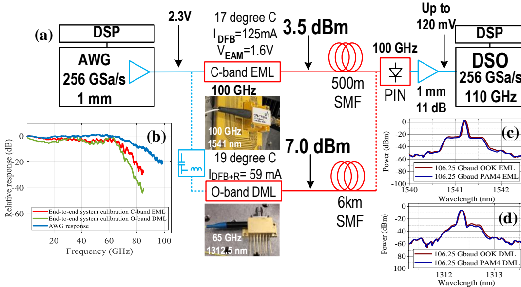
Fig. 1. (a) Experimental setup. (b) Calibrated end-to-end system amplitude responses for both EML and DML configurations. (c). The optical spectra of modulated EML. (d) The optical spectra of modulated DML.
